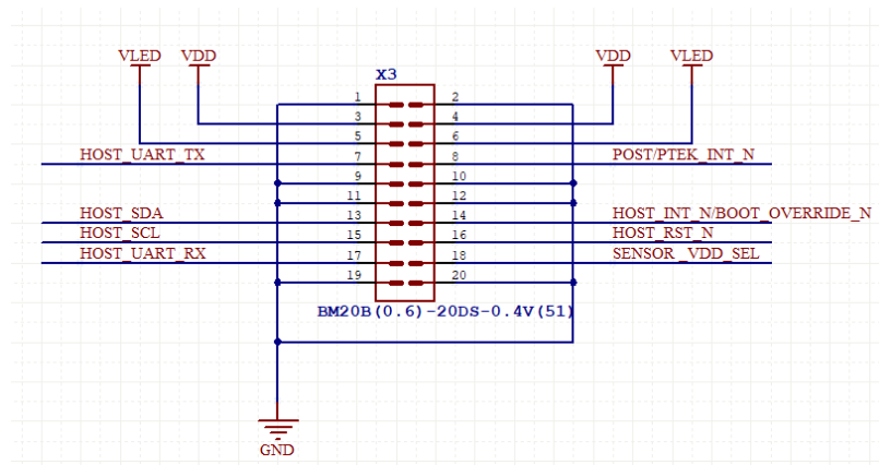
Figure 4: Benchmark Wrist 1.4 Connector
