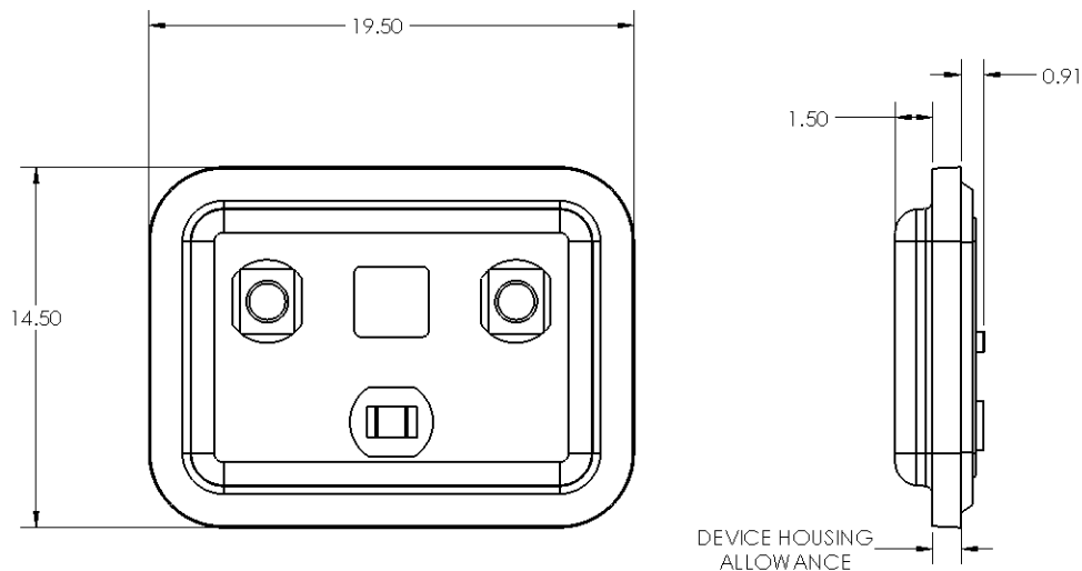
Figure 6: BW 1.4 Sensor Module Preliminary Drawing
